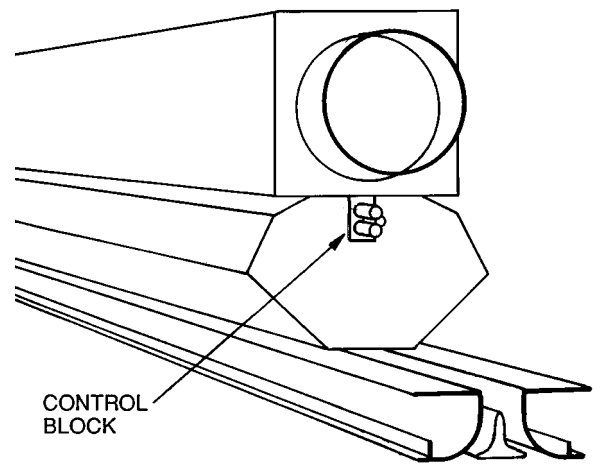
Fig. 12 — Control Block
